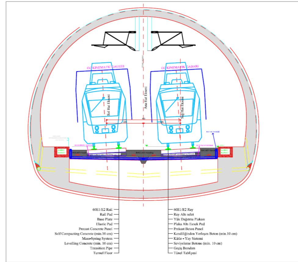
Rail Track Tunnel Section with no Ballast and with Cant
