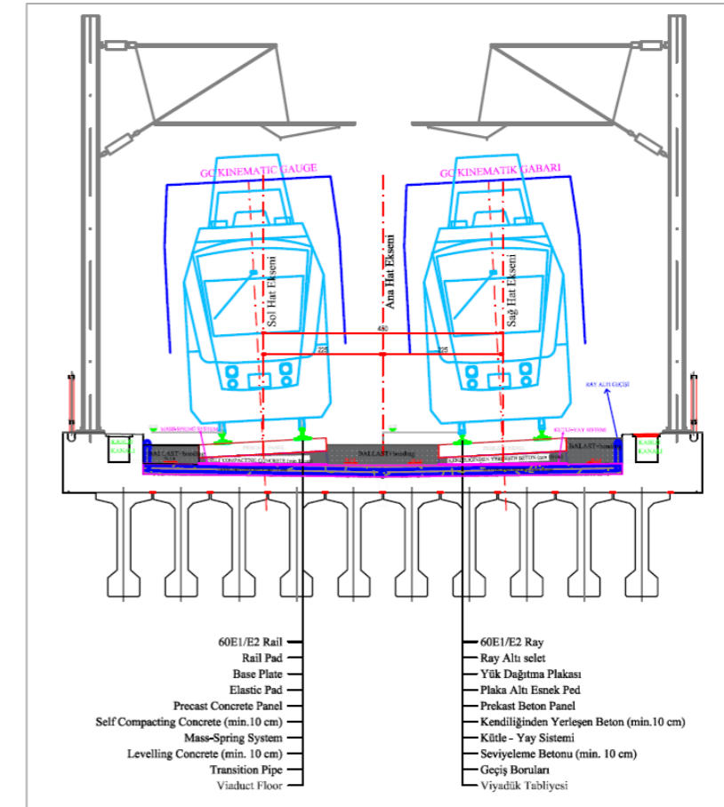
Rail Track Viaduct Section with Cant and no Ballast
