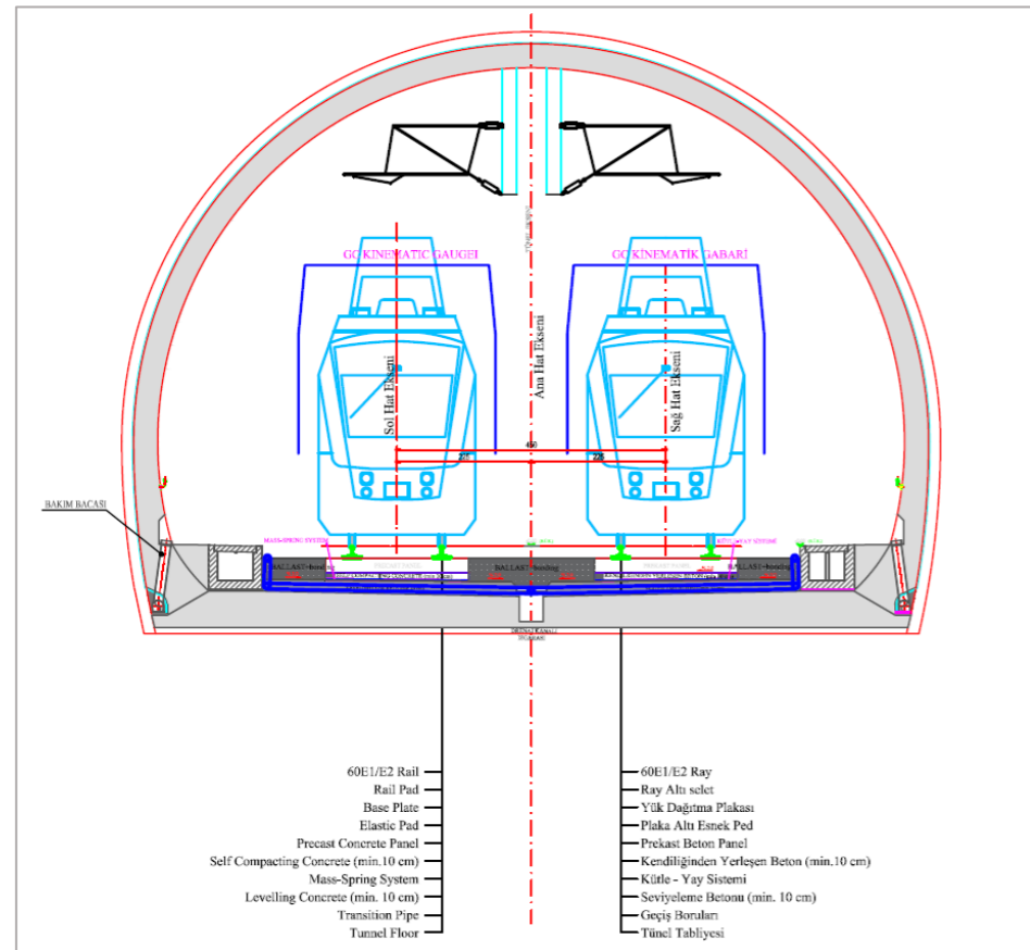
Rail Track Tunnel Section with Base Slab, no Ballast and no Cant
