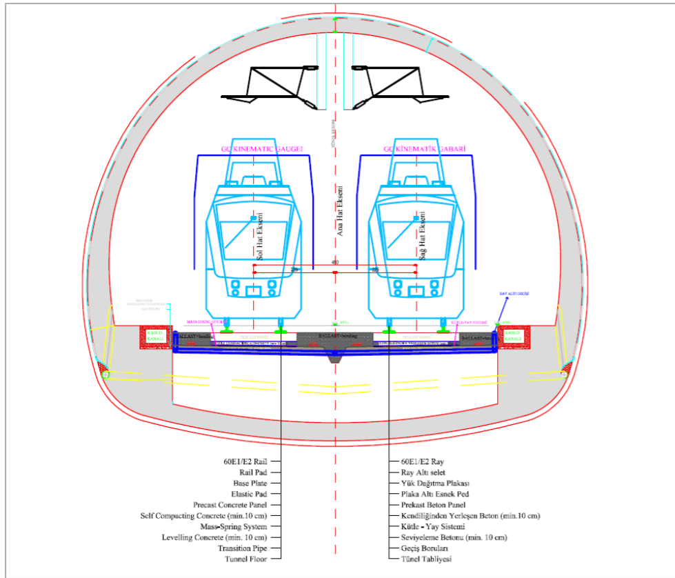
Rail Track Tunnel Section with no Ballast and no Cant
