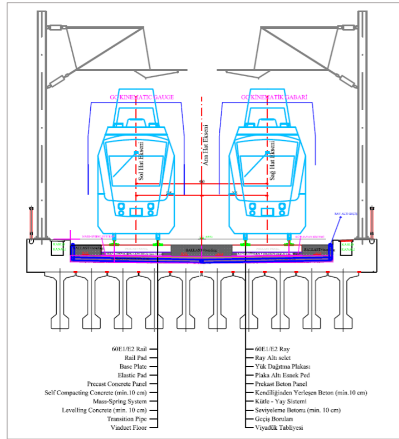
Rail Track Viaduct Section with no Cant and no Ballast
