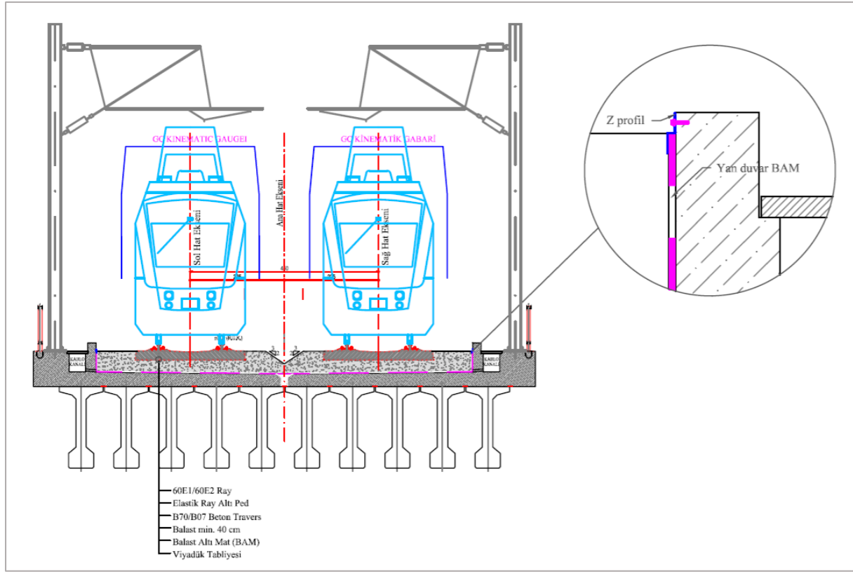
Ballasted Rail Track Viaduct Section with no Cant
