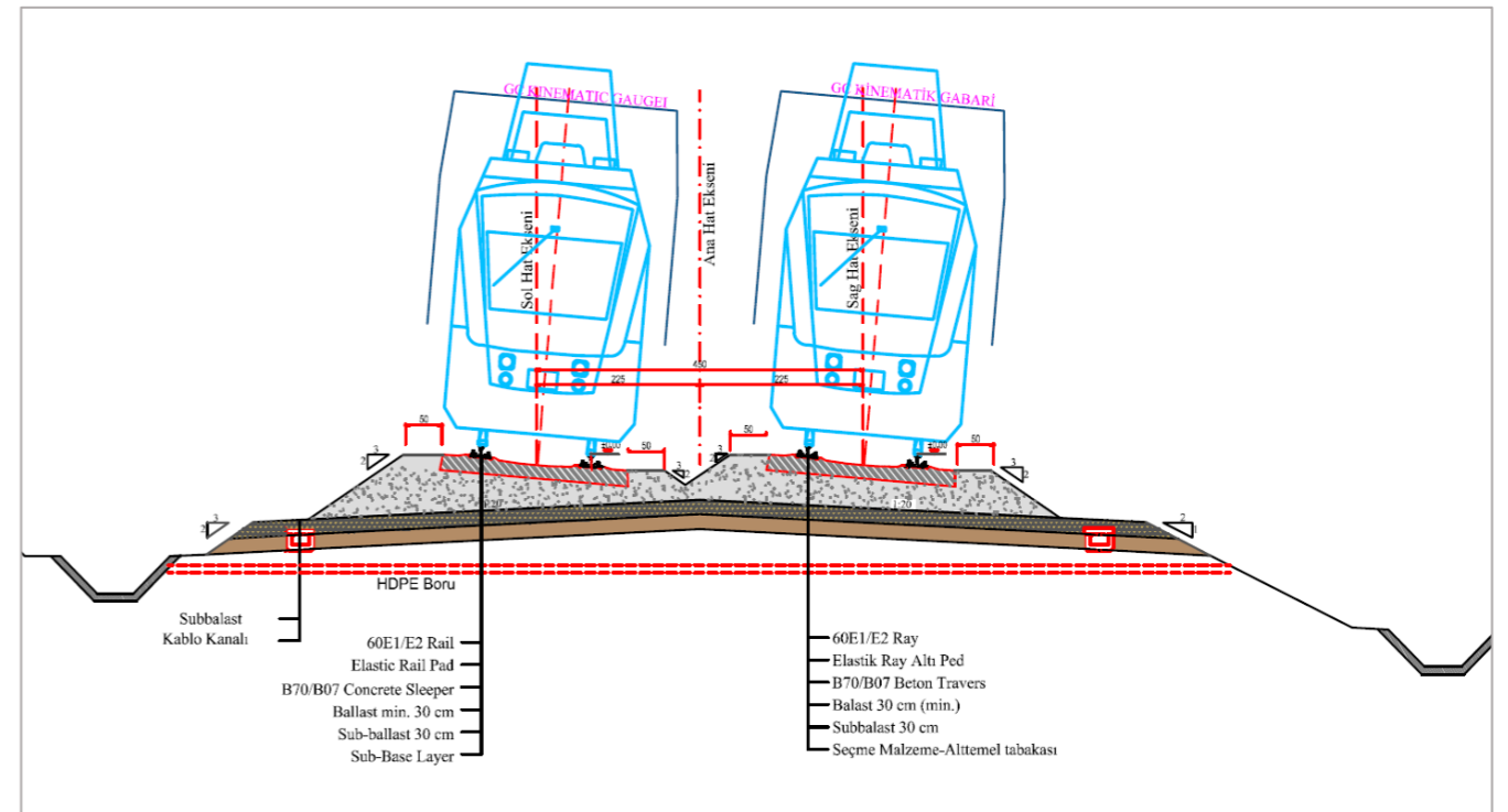
Ballasted Rail Track Section with Cant, no Catenary
