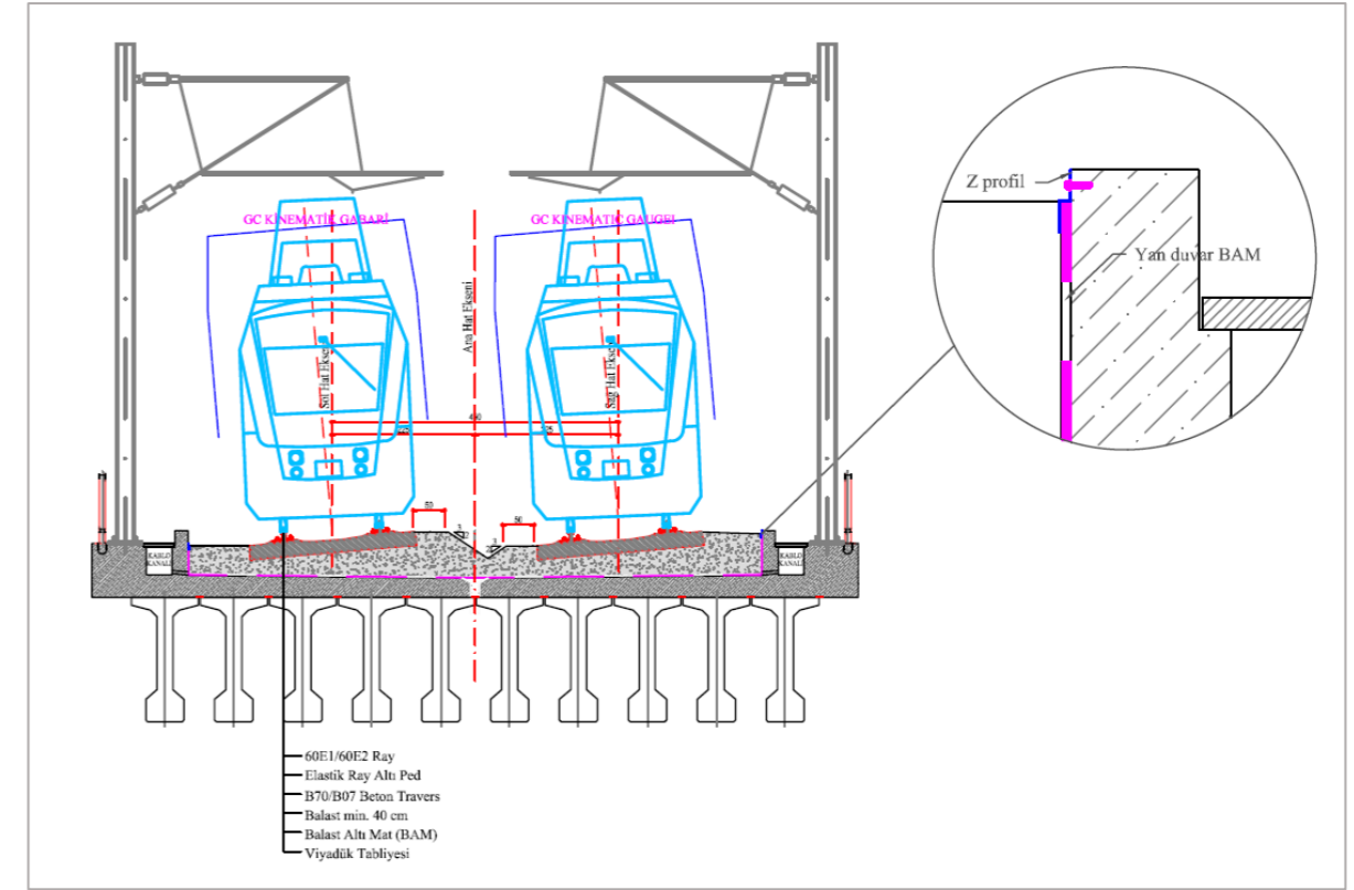
Ballasted Rail Track Viaduct Section with Cant
