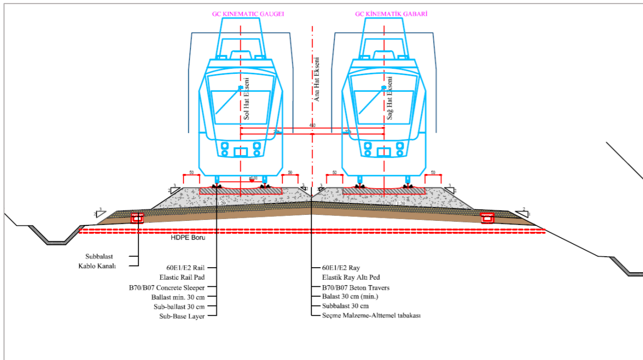
Ballasted Rail Track Section with no Cant, no Catenary
