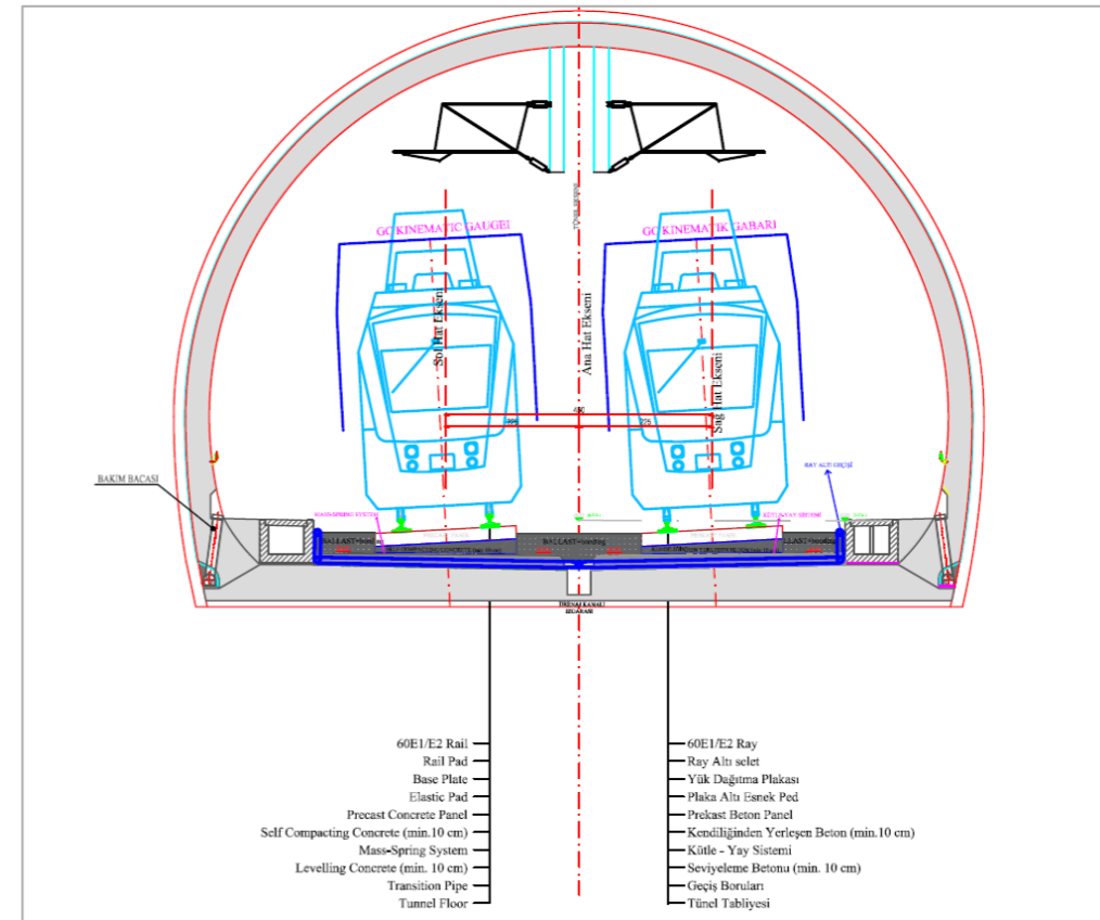
Rail Track Tunnel Section with no Ballast and with Cant
