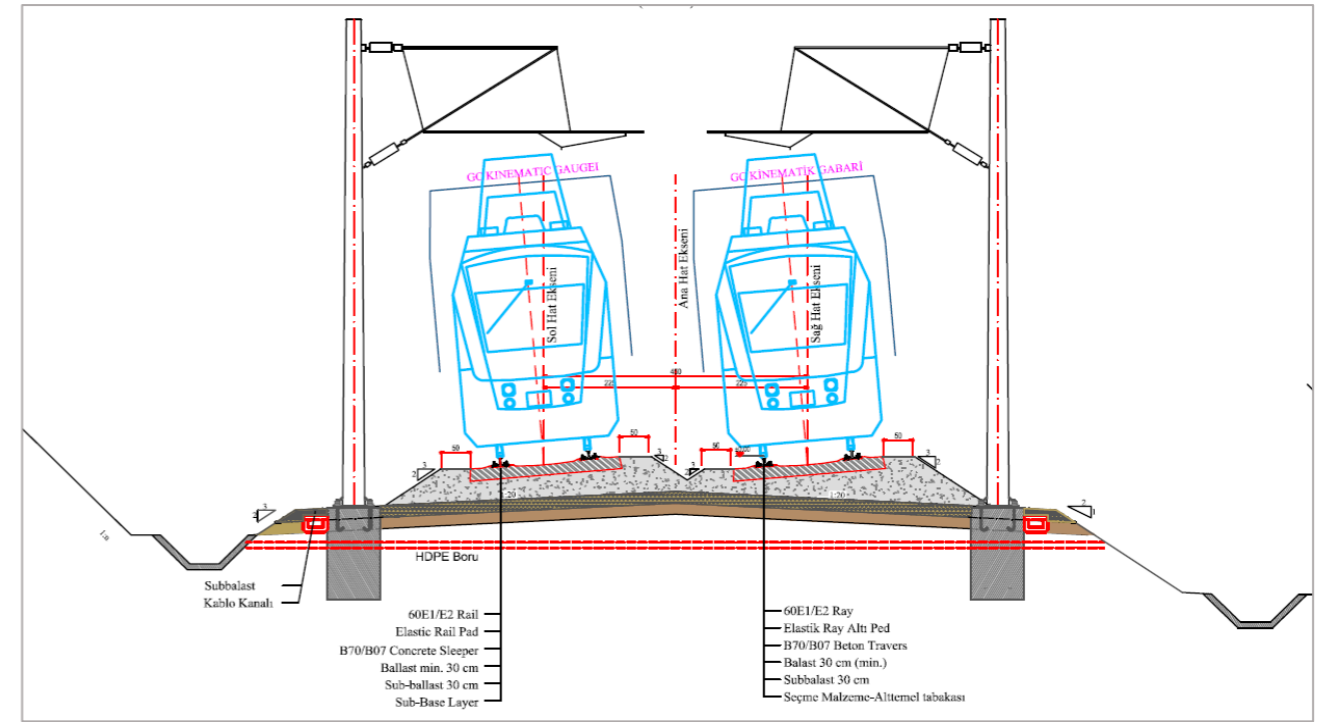
Ballasted Rail Track Section with Cant
