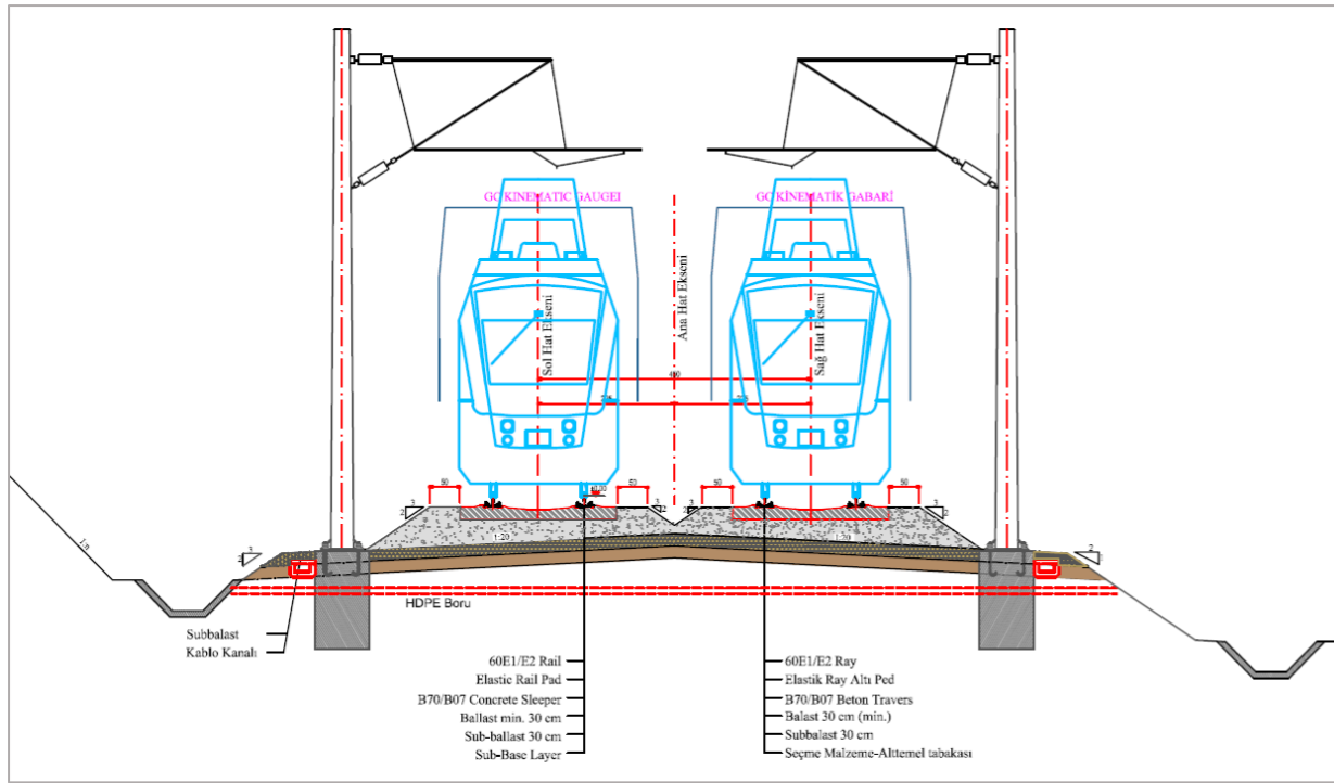
Ballasted Rail Track Section with no Cant
